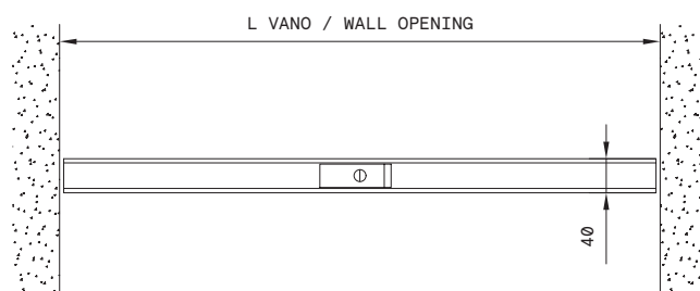
MECCANISMO CENTRALE / CENTRAL MECHANISM
