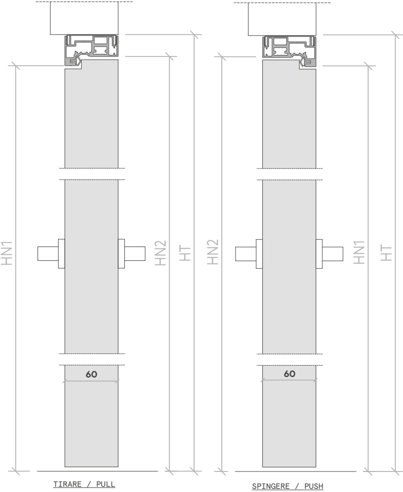
V3 2100 × 800 misure in mm V3 2100 × 800 measures in mm
